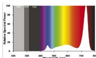
Gro-Lux® LED E27 Vegetative
