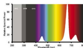
Gro-Lux® LED E27 Flowering
