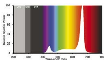
Gro-Lux® LED E27 Far-Red
