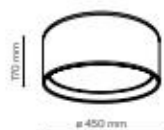
3376 / BILBAO 4 x E27 / 230V / max 15W / LED AB / 9242 / 9246 / 9244
