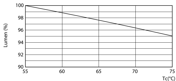
LEDtube HF 1200mm HO-UO 14-16W G13 830-865 T8
