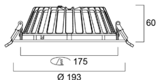
Insaver Slim 175
