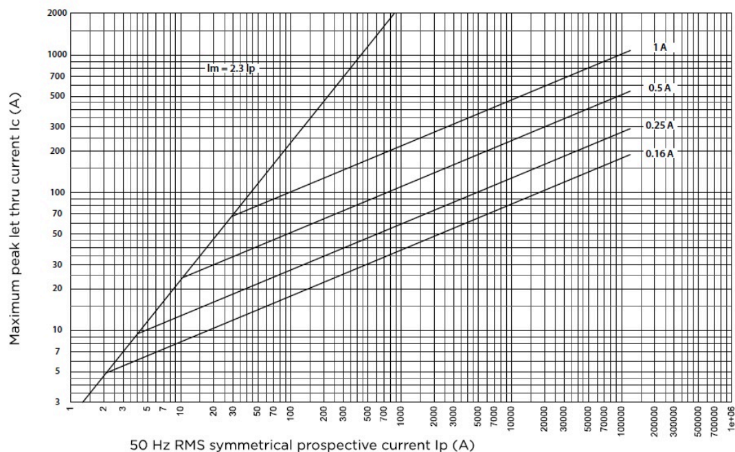
Cut-off current characteristics, CH10 aM
