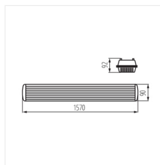
MAH PLUS-158/4LED/PC
