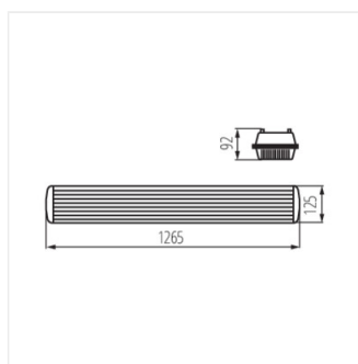
MAH PLUS-236/4LED/PC
