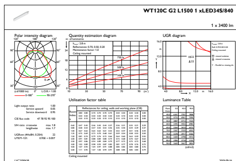
IFGU1_WT120CG2L15001xLED34S840
