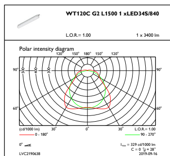
OFPC1_WT120CG2L15001xLED34S840
