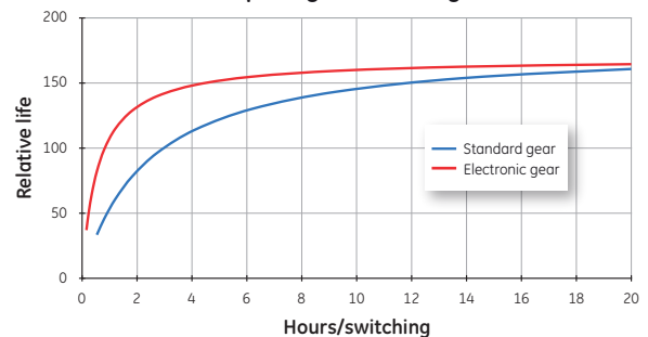
Life versus frequency of switching
