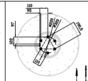
Rundo ø850
