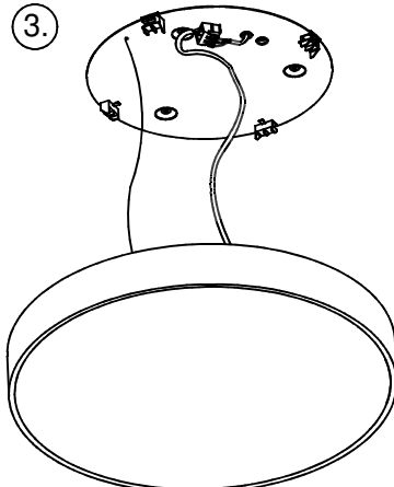
Rundo ø850
