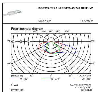
OFPC1_BGP292T251xLED120-4S740DM11W
