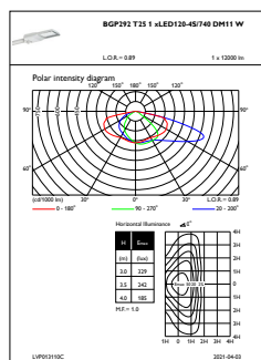
OFPL1_BGP292T251xLED120-4S740DM11W
