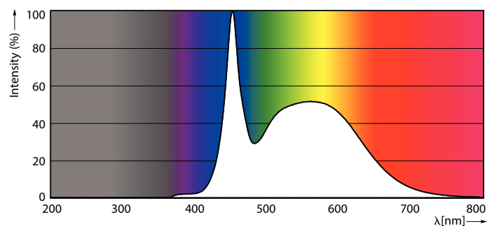
CorePro LEDbulb 40W E27 865 FR A60
