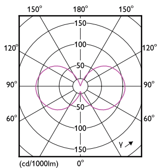
LEDbulb MAS A60 7,8W E27 927 CL-LDD
