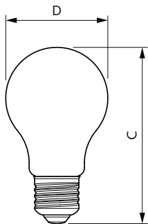
MASTER VLE LEDBulb D7.8-75W E27 927 A60 CLG
