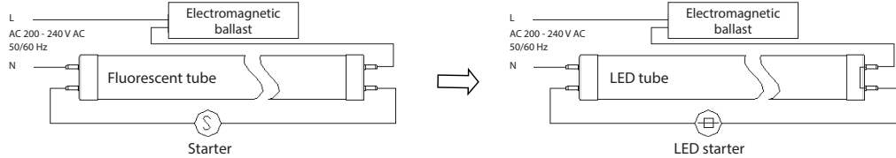
Figure No. 1 - switch off the power supply. Figure No, 2+3 - remove the old fluorescent tube. Figure No. 4 - switch off the power supply. Figure No. 5 - remove the LED starter (included). Figure No. 6 - insert the LED tube Figure No. 7 - turn the tube by 90°. Figure No. 8 - switch on the power supply and check the direction of radiation.
