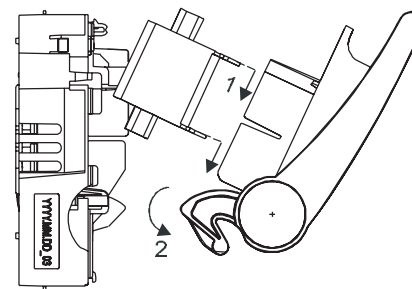
XLP00 1/2/4-pole: Padlock facility
