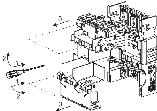
XLP00 3-pole: Remove the upper and lower terminal cover
