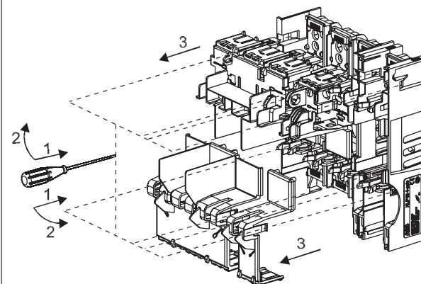
XLP00 1/2/3/4-pole: Install fuse and front cover
