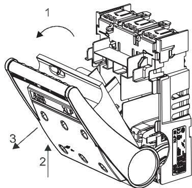
XLP00 3-pole: Remove the front cover
