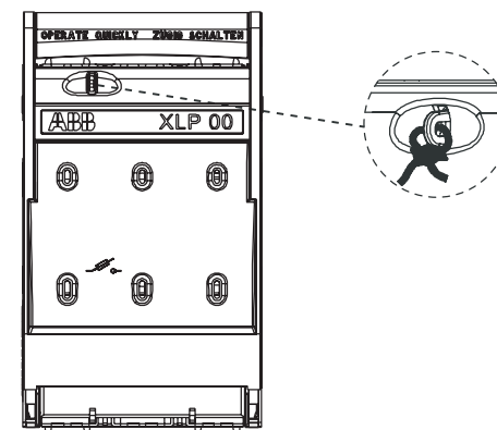
XLP00 3/4-pole: Sealing facility
