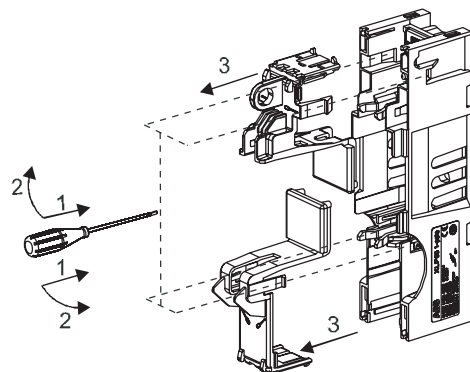
XLP00 2-pole: Remove the upper and lower terminal cover
