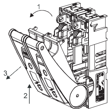
XLP00 3-pole: Remove the front cover
