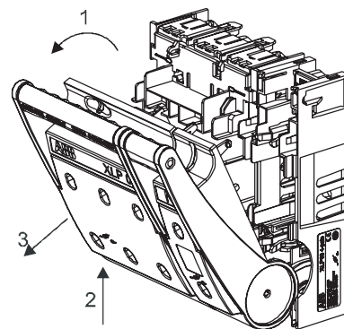
XLP00 1/2/3/4-pole: Install fuse and front cover
