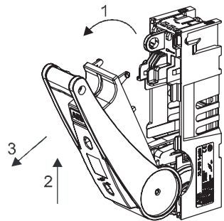
XLP00 2-pole: Remove the front cover
