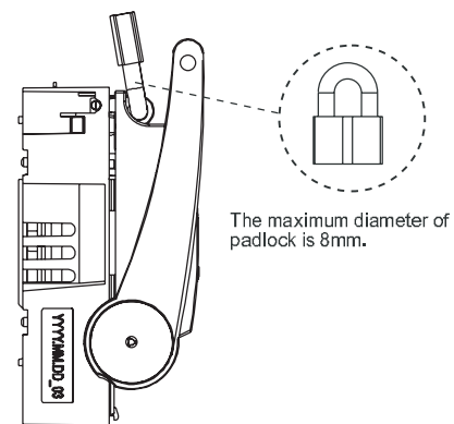
XLP00 1/2/4-pole: Padlock facility
