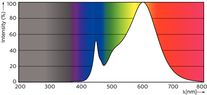
LEDtube 100mm 5W G24D-1 830 475lm
