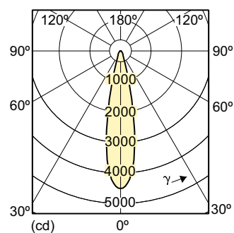
LDLD_CDM-Rm_20W_25D_0003-Light distribution diagram
