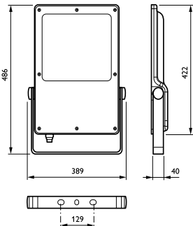
BVP130 LED260-4S/740 PSU S ALU C1KC3 T35
