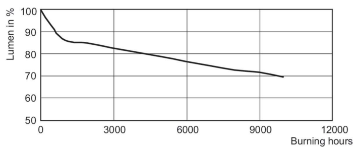
LDLM_CDM-Tm_35W_930_PGJ5-Lumen maintenance diagram
